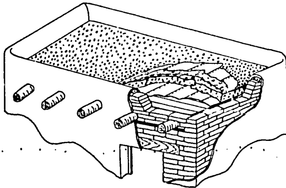
Figure 85. The cutaway section of this bunker fill roof shows the layered structure of the roof. From the top down, the components are gravel and asphalt, building paper, earth fill, building paper, wood sheathing and supporting beams (vigas).
