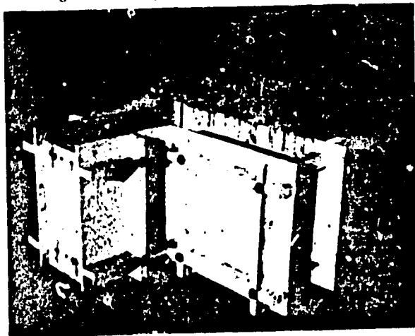
Figure 74. Plywood corner form for rammed earth walls.
