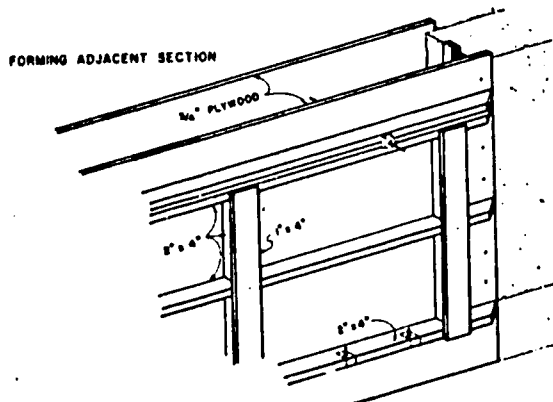
Figure 76. This is a special form that was designed to use the metal tie strips shown in Figure 75.
