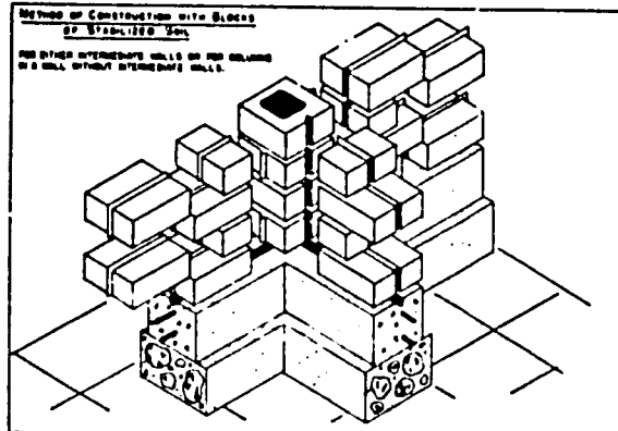
Figure 49. The various shapes of blocks produced by the Landcrete block-making machine allow rapid construction of corners and tees.
