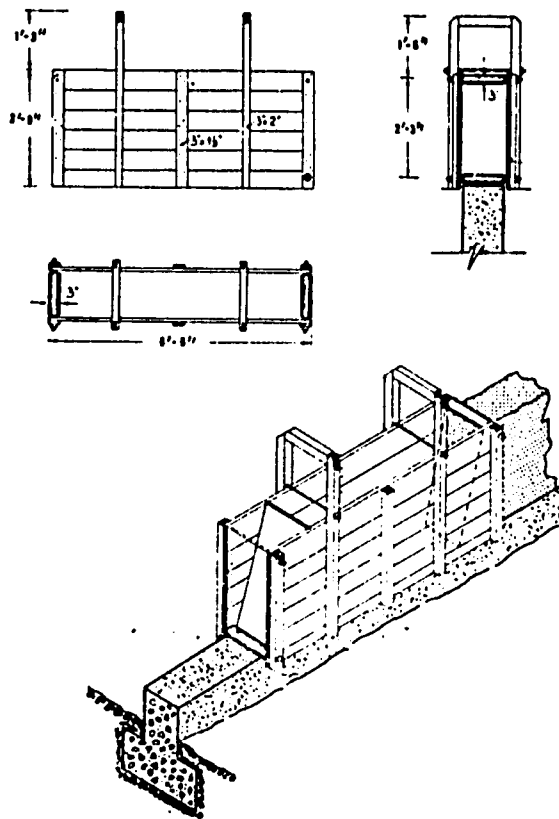
Figure 77. Form for ramming.
