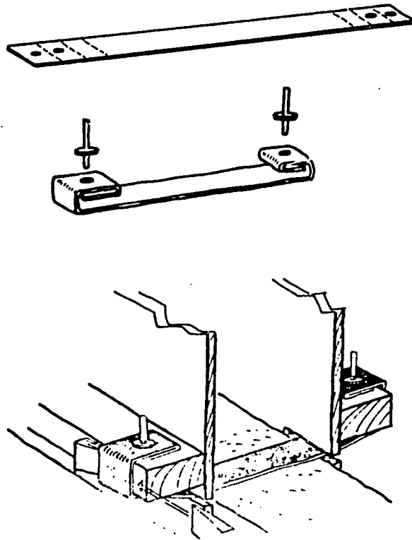
Figure 75. Thin metal strips such as these can be used instead of bolts to tie rammed earth forms together.
