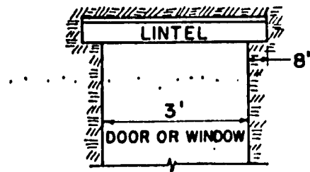
Figure 95. Wood lintel.
