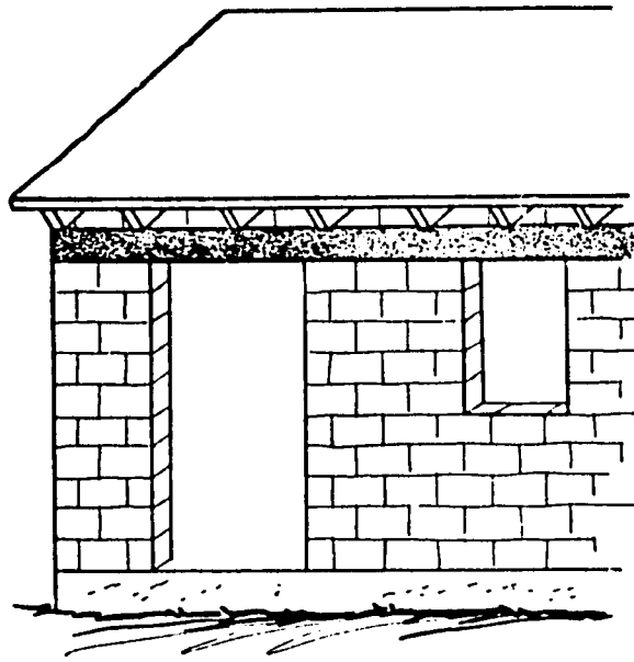
Figure 10. This shows a combination bond beam and lintel, made from reinforced concrete, that can be used, on low-ceiling houses.
