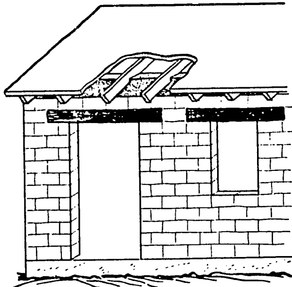
Figure 68. This shows how timber lintels are used above doors and windows. Above the lintels (in the cut-out section) is shown a concrete bond beam.
