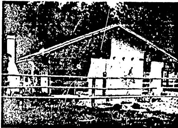
Figure 3. Machine-made blocks form the walls of this house.
