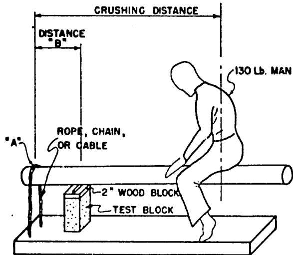
Figure 15. Simple lever test for determining strength of blocks (see Table 2).
