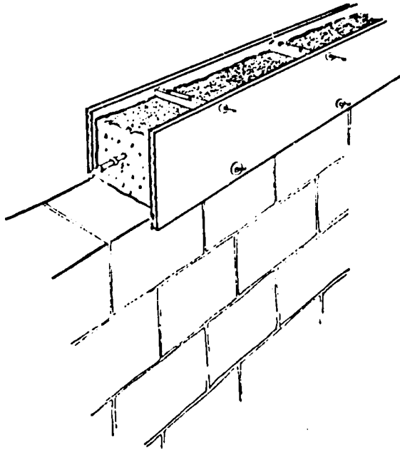
Figure 71. Forms like this can be used to pour concrete bond beams and lintels in place in the wall.
