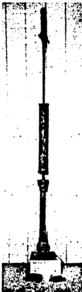
Figure 79b. Assembled sliding weight tamper.
