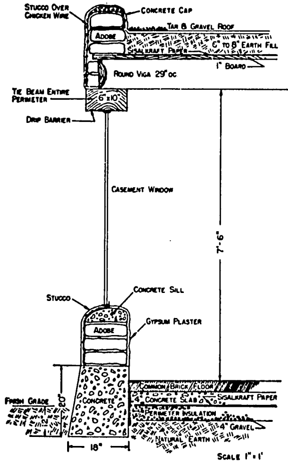
Figure 65. This typical wall section for adobe is used by a well known Albuquerque, N. M., adobe building contractor.
