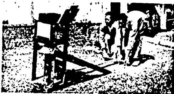
Figure 51. The compression and ejection stroke with this Ellson block-making machine consumed 1.4 seconds by stop watch.
