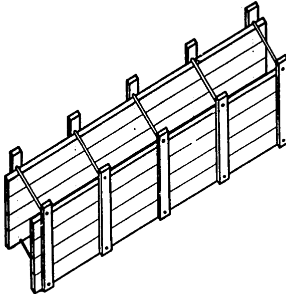
Figure 72. Form for ramming.
