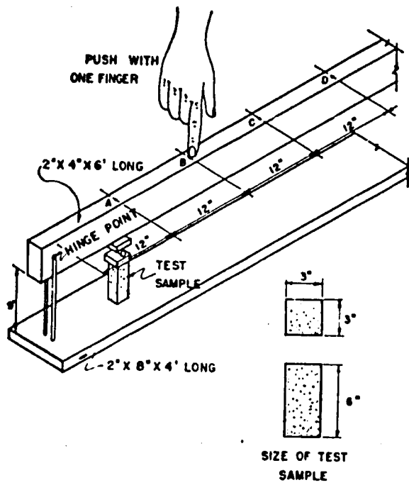
Figure 94. Simple lever tester for soils.
