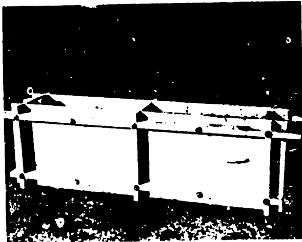
Figure 73. Straight form for rammed earth walls.
